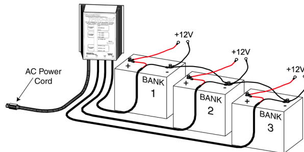
Common Negative, three 12V battery banks
